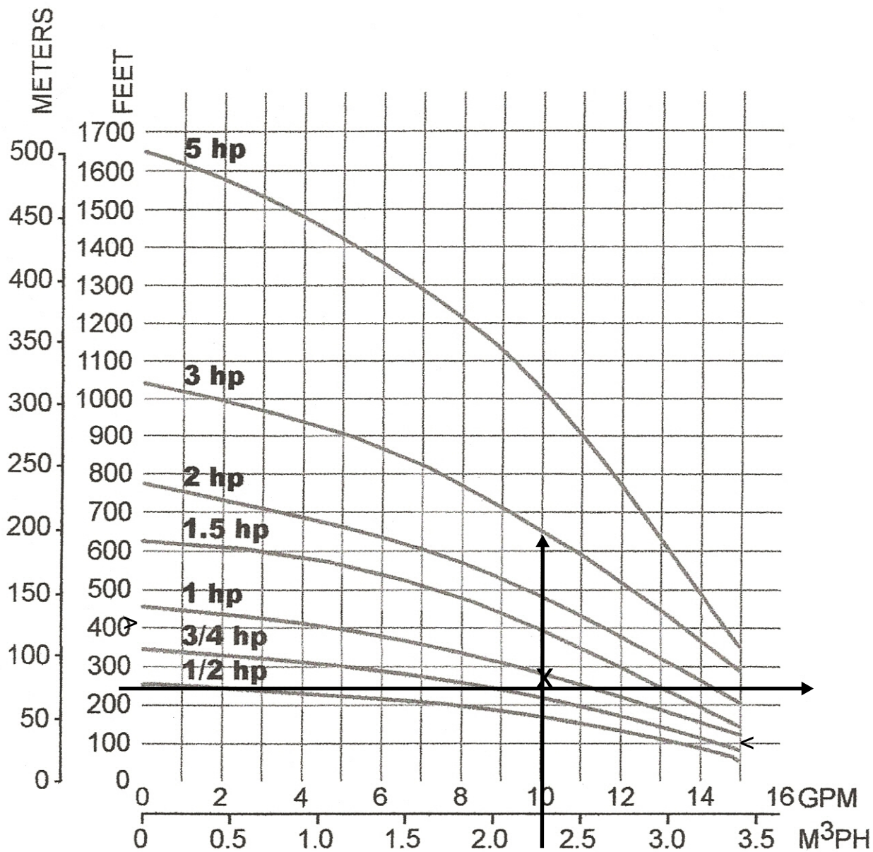
Franklin 1HP 10GPM Selection
